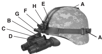
FIGURE 3-2. ATTACHING ATN PS-15 TO HELMET MOUNT
